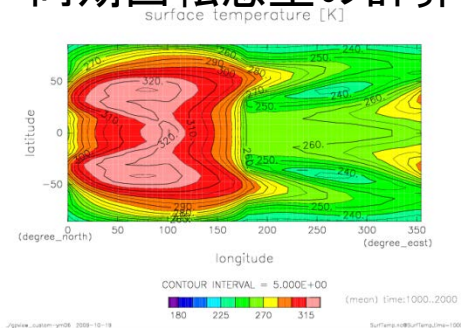
Time mean Surface temperature, T21L16
